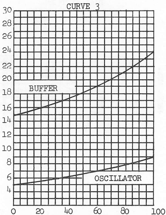
DIAL SETTINGS EXCITER CALIBRATION 16.6-23 MC POSITION
