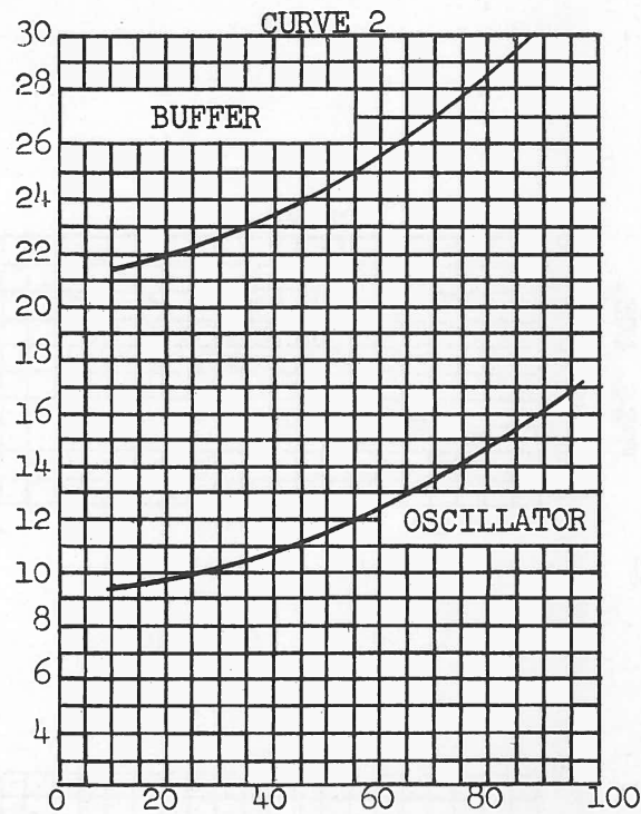
DIAL SETTINGS EXCITER CALIBRATION 23-30 MC BANDSWITCH POSITION VIKING II-CDC TRANSMITTER
