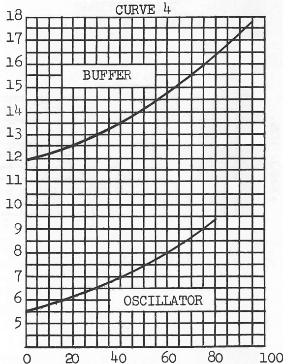
DIAL SETTINGS EXCITER CALIBRATION 11.7-16.6 MC POSITION
