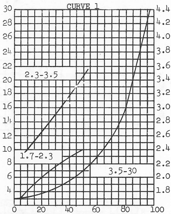
FINAL DIAL SETTING FINAL AMPLIFIER TUNING CALIBRATION VIKING II-CDC TRANSMITTER
